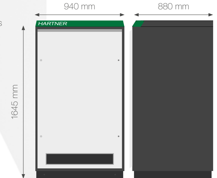
TM 426 Expansion unit | Front and side view
