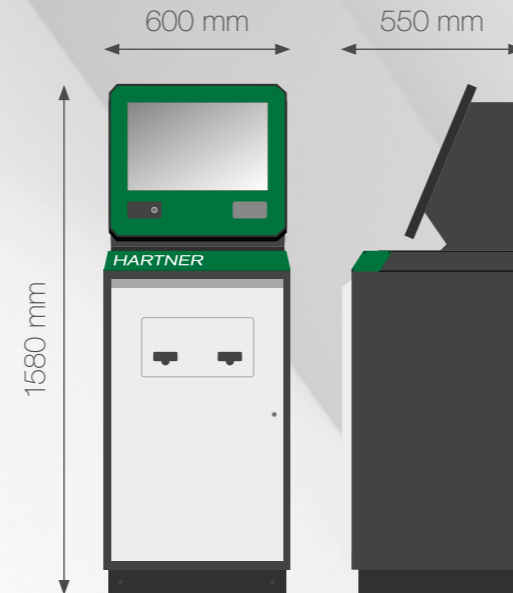
TM 426 Base unit | Front and side view
