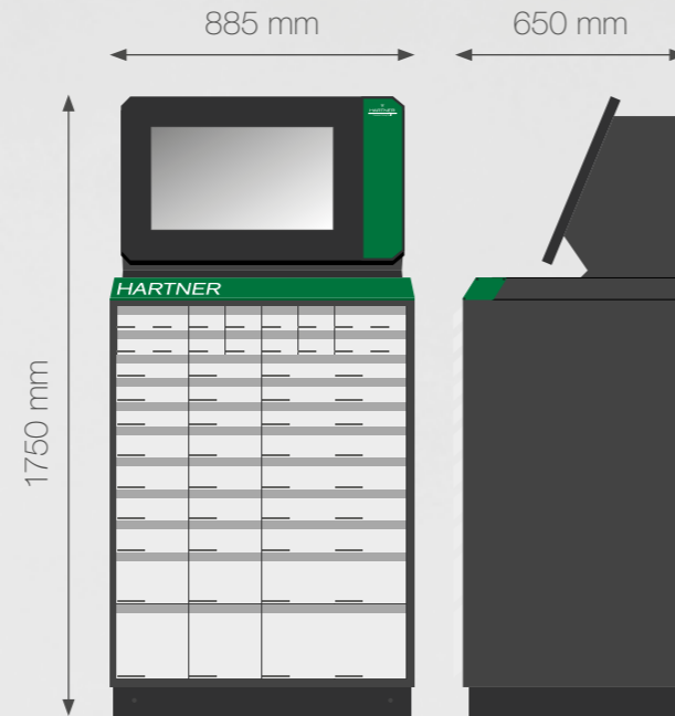
TM 326 Base unit | Front and side view
