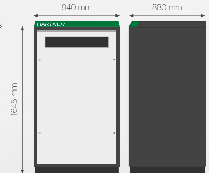
TM 426 Expansion unit L | Front and side view
